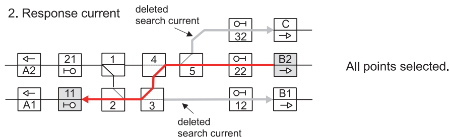
Figure 3.15 Geographical interlocking
