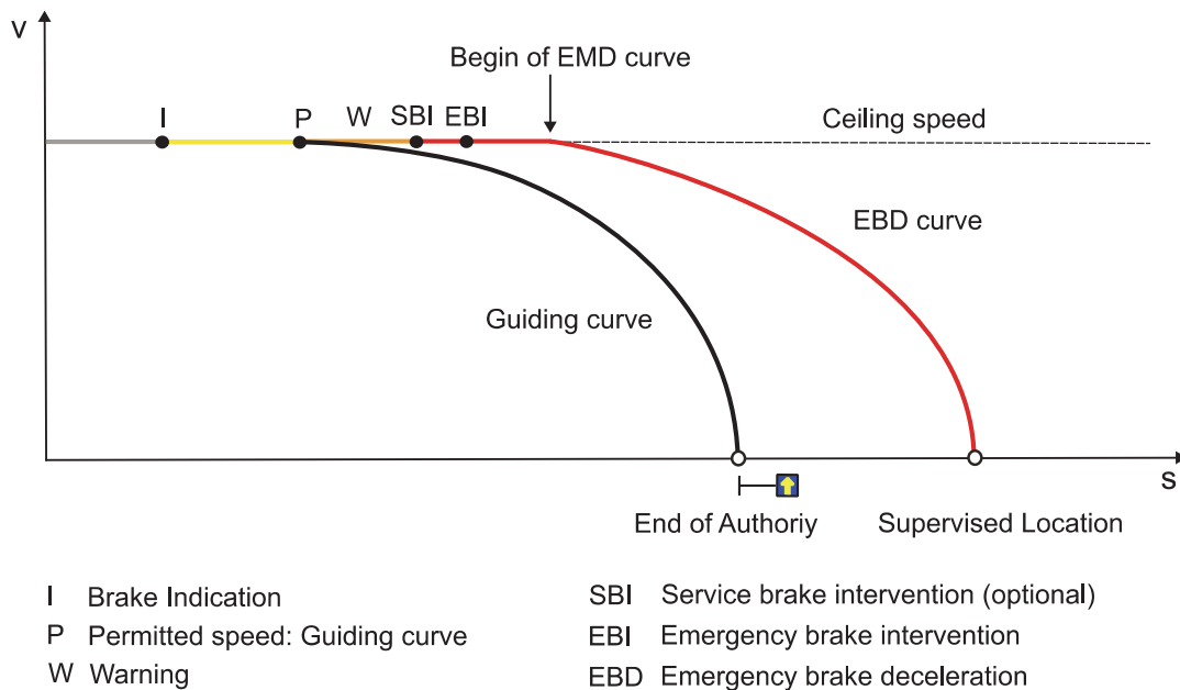
Figure 4.8 Guiding and supervision principle in ETCS Level 2
