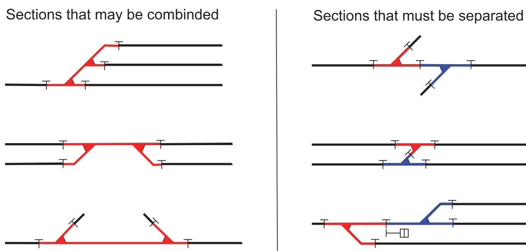
Figure 3.13 Combining and separating track sections of adjacent points
