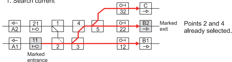
b) Route setting principle (example: 11-B2)
