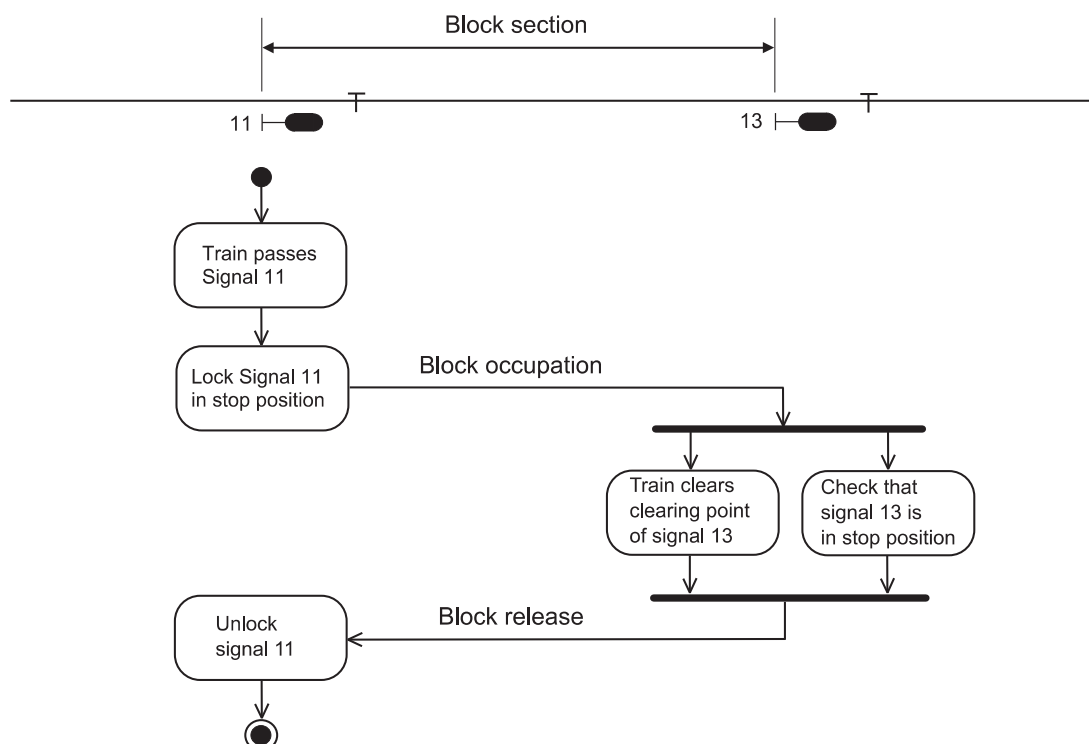
Figure 2.13 Block protection of following movements
