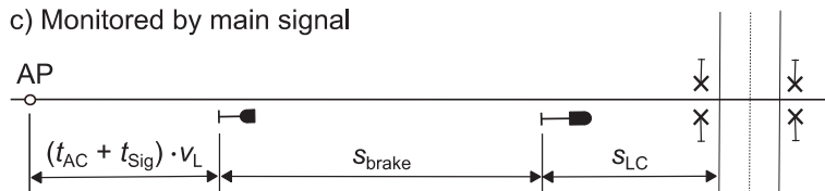
Figure 5.2 Calculation of the initiation section
