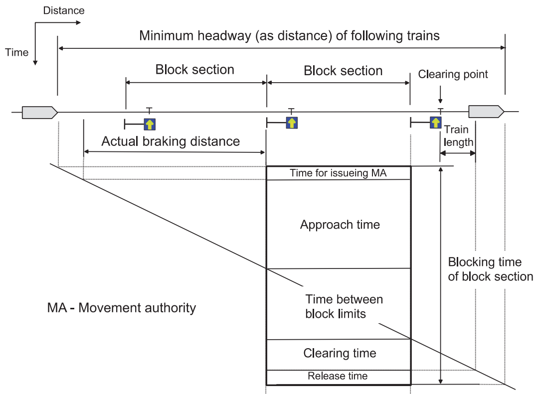
Figure 2.11 Blocking time of a block section on a cab signalling line
