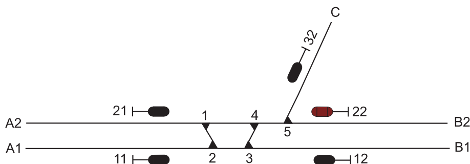
Figure 3.14 Infrastructure example
