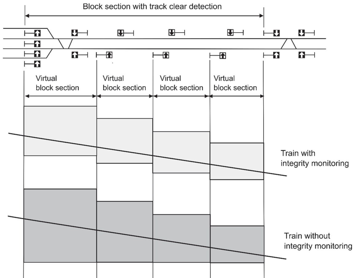
Figure 4.9 Blocking time stairways in ETCS Level 2 HD with virtual block
