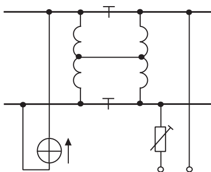
Figure 1.7 Impedance bonds
