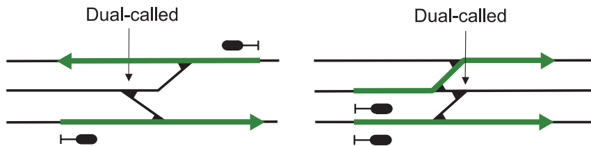
Figure 3.8 Dual-called points
