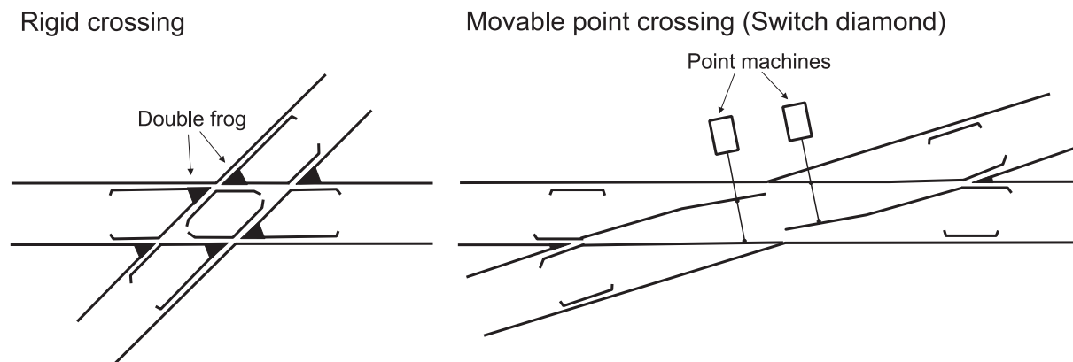
Figure 1.3 Crossings
