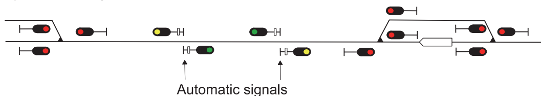
b) Opposing signals held down by traffic locking
