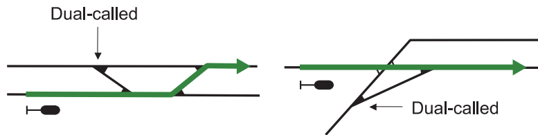
Figure 3.9 Self-selective protective points
