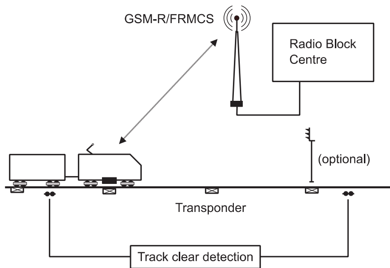
Figure 4.4 ETCS level 2 without train integrity monitoring
