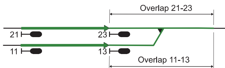
Figure 3.11 Shared overlaps
