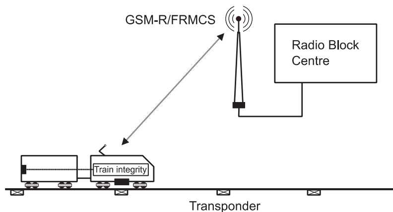
Figure 4.6 ETCS Level 2 with train integrity monitoring
