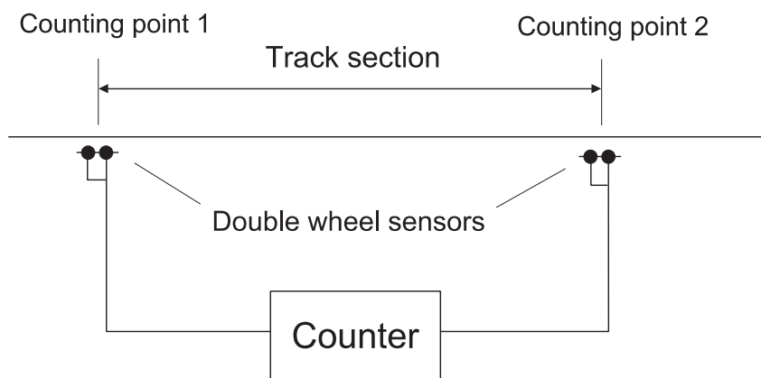
Figure 1.9 Axle counter
