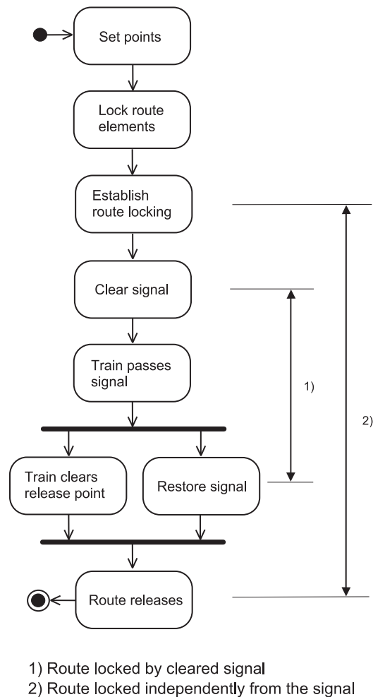
b) Route locking procedure without approach locking (German route locking principle)
